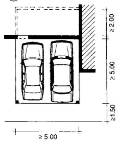
⑪ Two cars, room for bicycles
