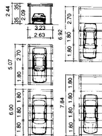
⑬ Individual carports (Osma/Gard)
