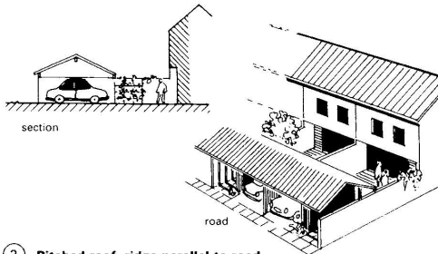
② Pitched roof, ridge parallel to road
