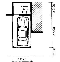
⑩ Carport for one car and bicycles
