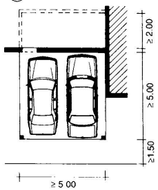
⑪ Two cars, room for bicycles
