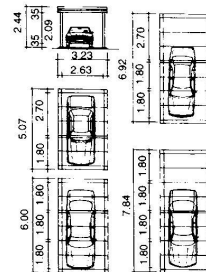
⑬ Individual carports (Osma/Gard)
