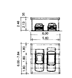
⑭ Double carports
