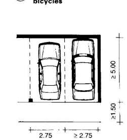
⑫ Common covered car-parking area
