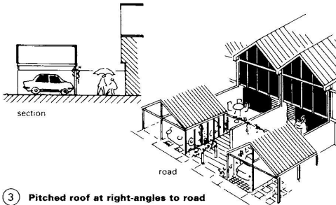
③ Pitched roof at right-angles to road
